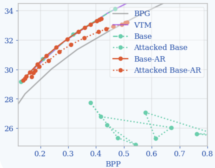
Kodak Attack-Resilient (PSNR)
