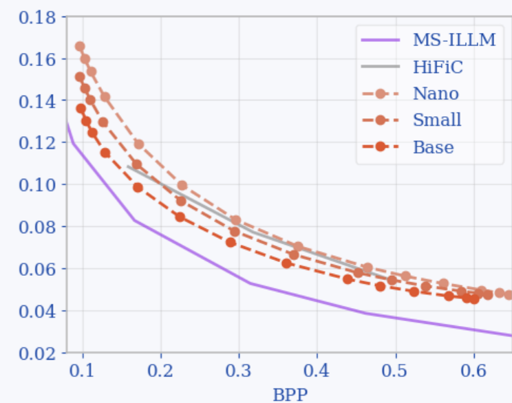
JPEG AI Compression (LPIPS)
