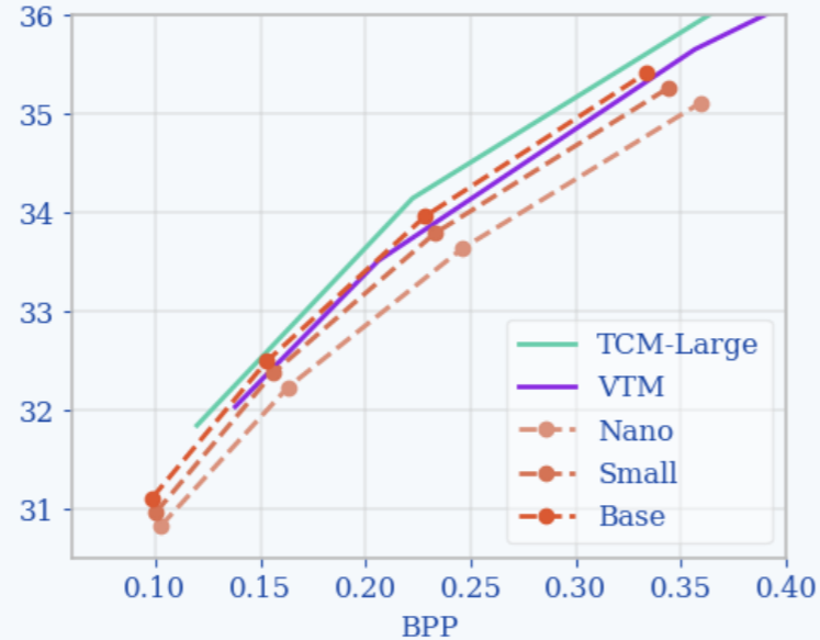
CLIC Compression (PSNR)
