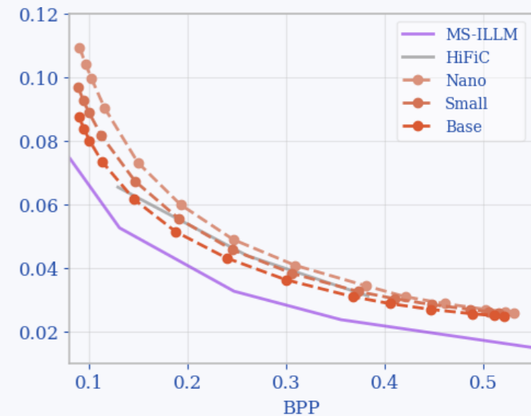
Tecnick Compression (LPIPS)
