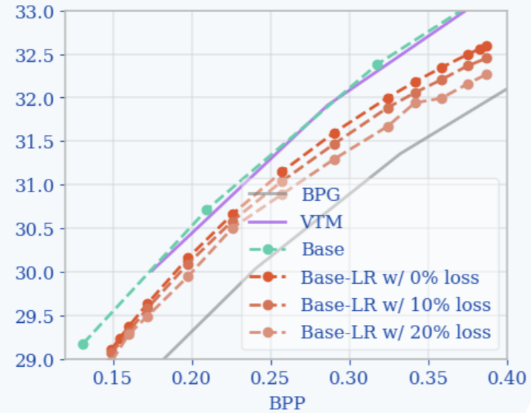
Kodak Loss-Resilient (PSNR)
