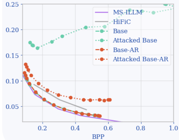
Kodak Attack-Resilient (LPIPS)
