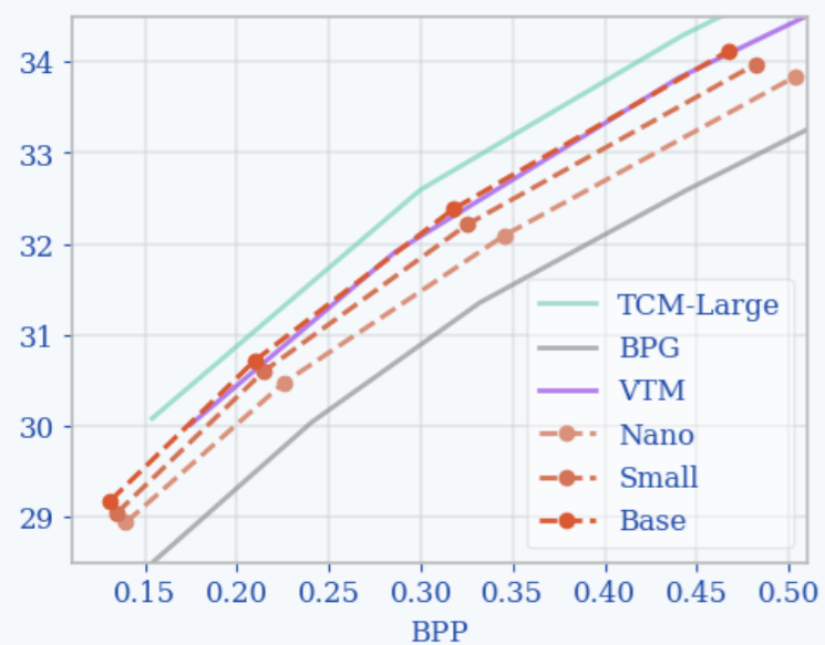
Kodak Compression (PSNR)
