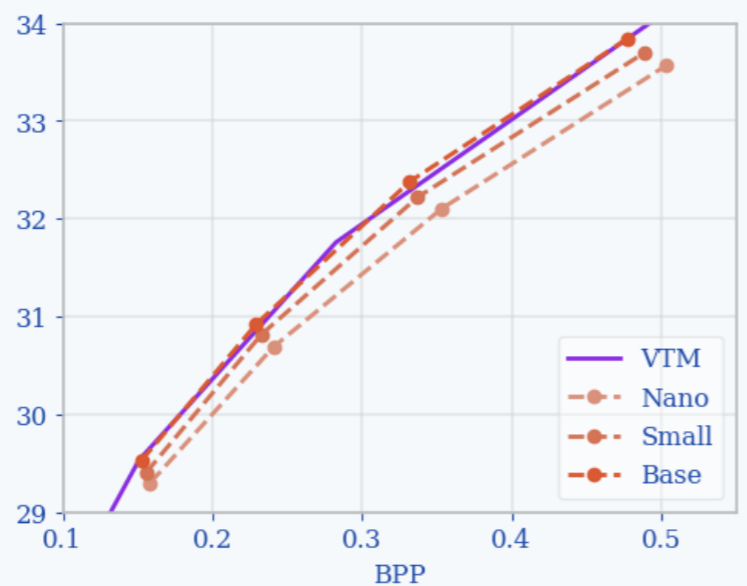
JPEG AI Compression (PSNR)
