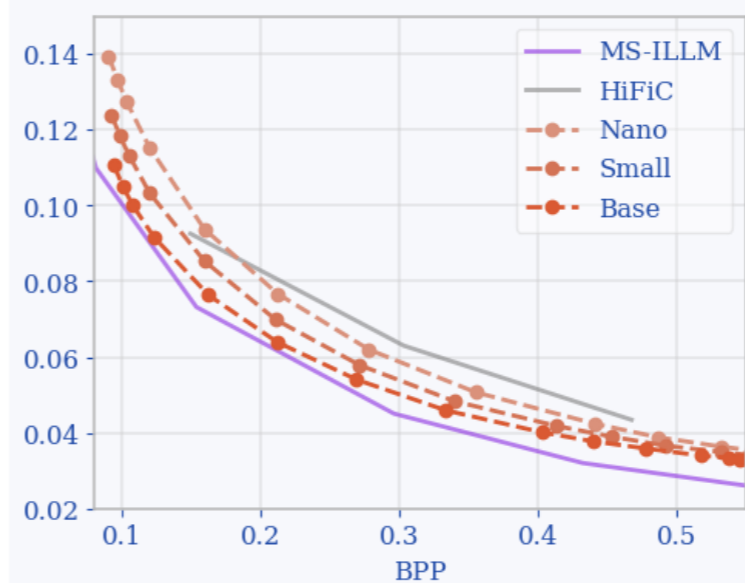
Kodak Compression (LPIPS)
