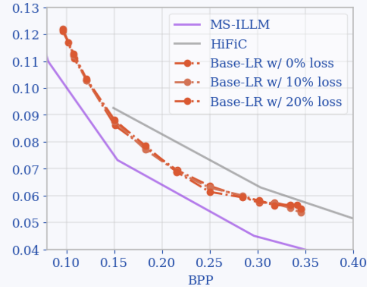
Kodak Loss-Resilient (LPIPS)
