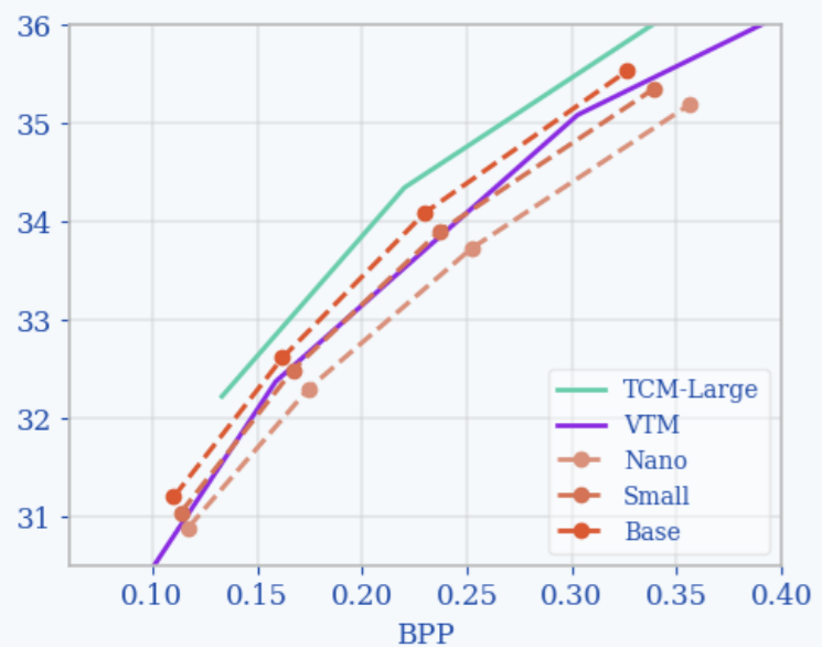
Tecnick Compression (PSNR)
